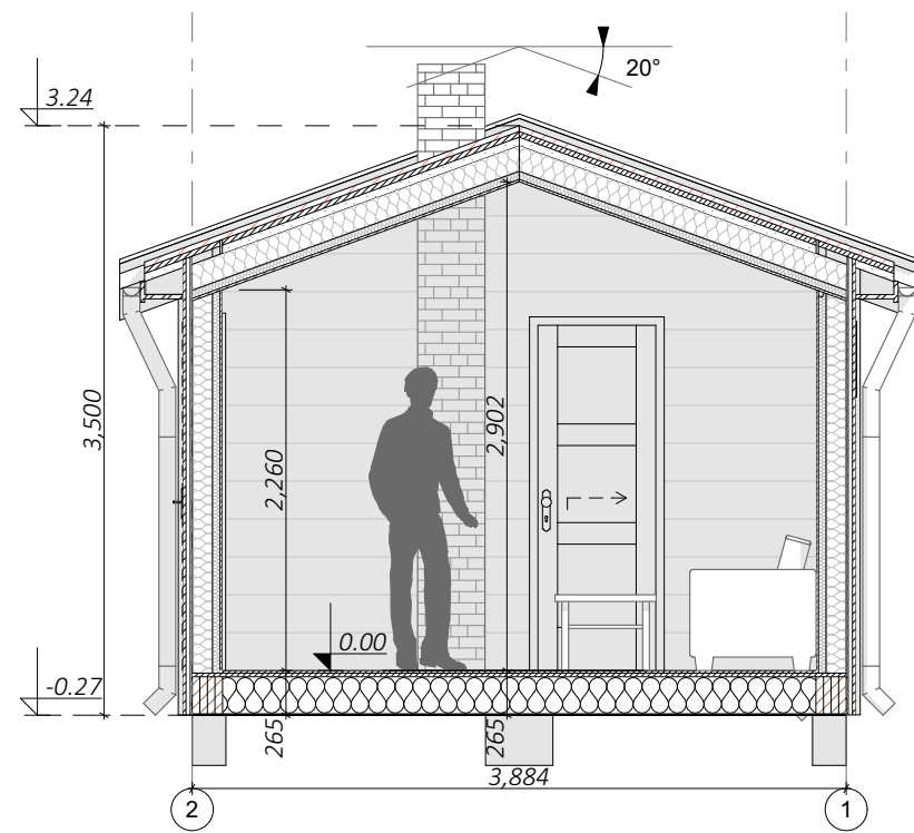
Section A - A S 1:50
