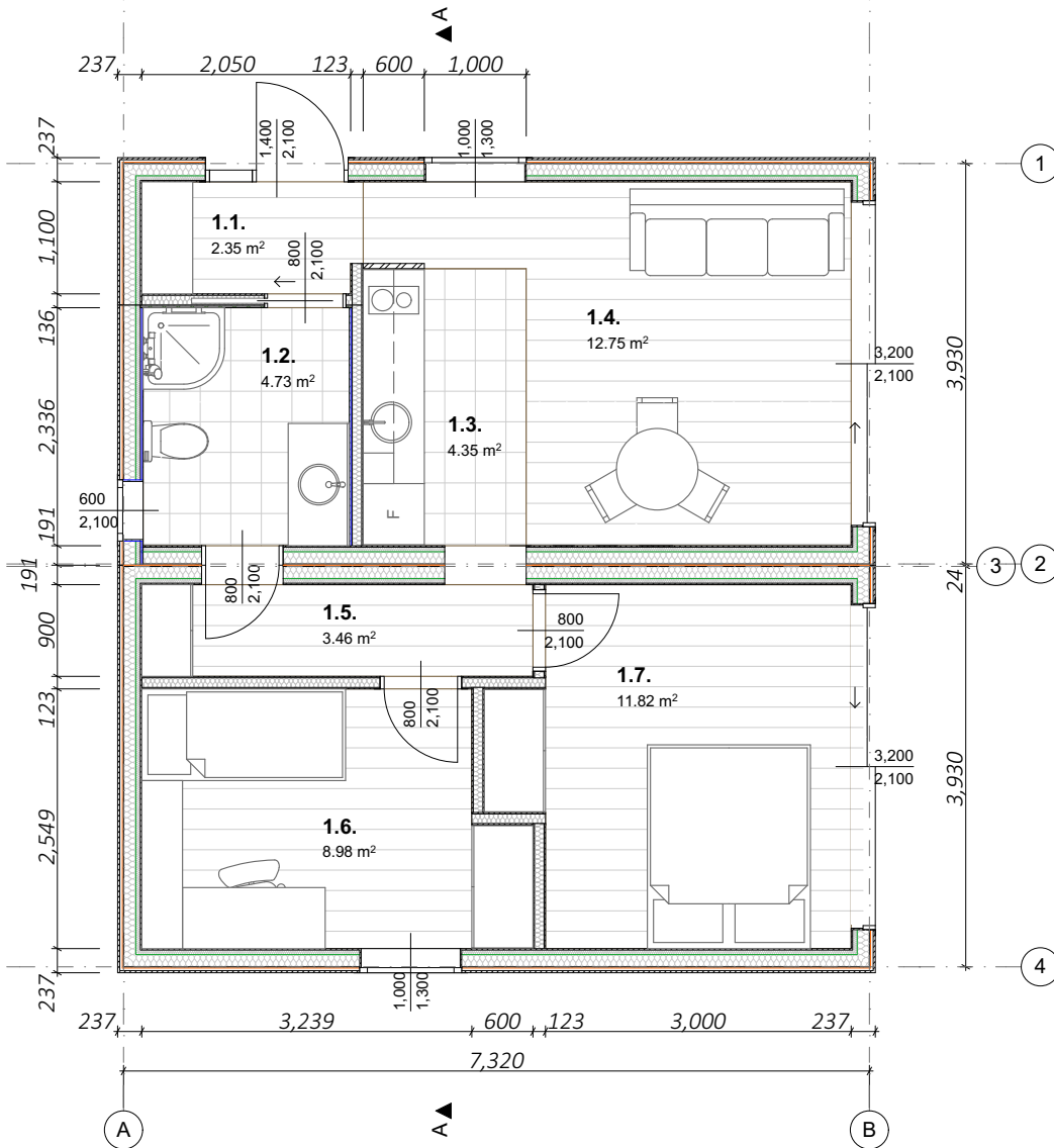
Floorplan S 1:75
